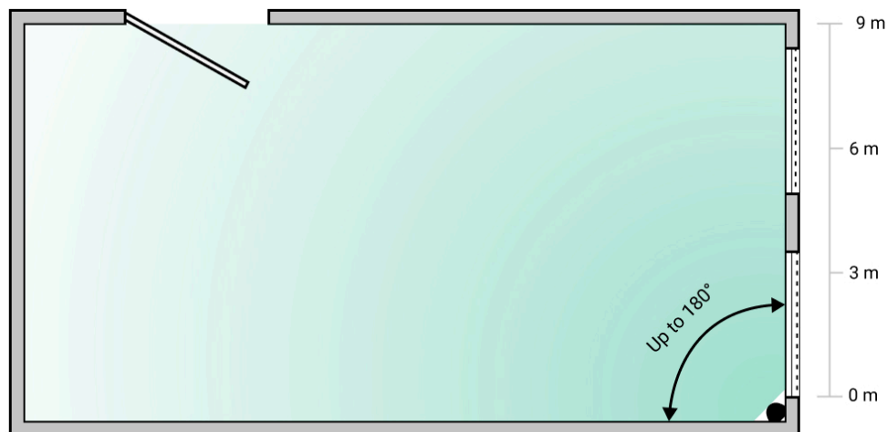
Detection angle of the glass break detector
